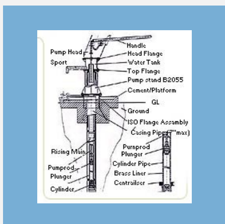
U3 Modified Deep Well Hand Pump
